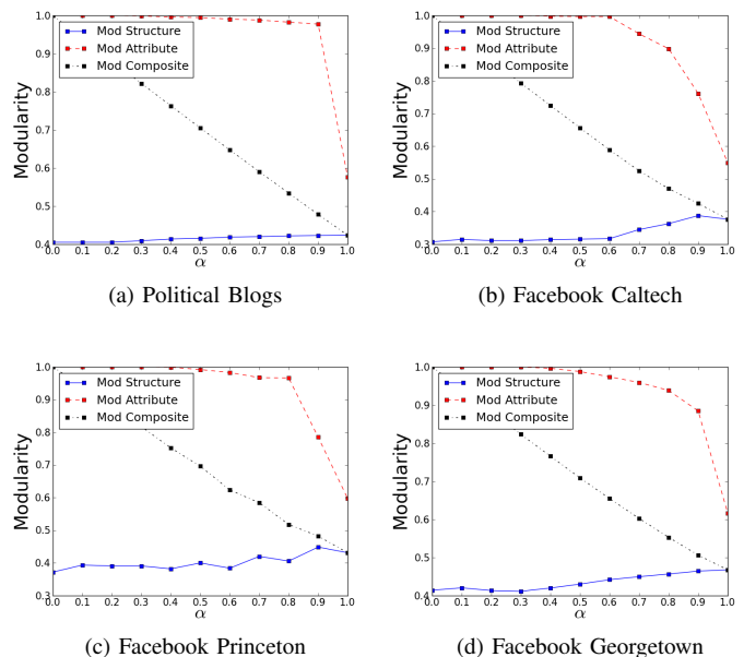
Figure 1: SAC1 modularity structure, modularity attribute and modularity composite for \alpha \in [0, 1]
