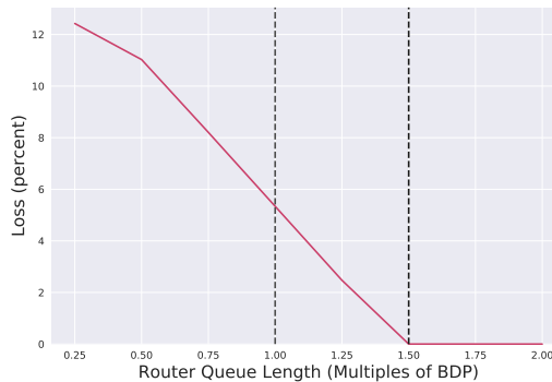
Figure 7. BBR's loss versus router queue size.
