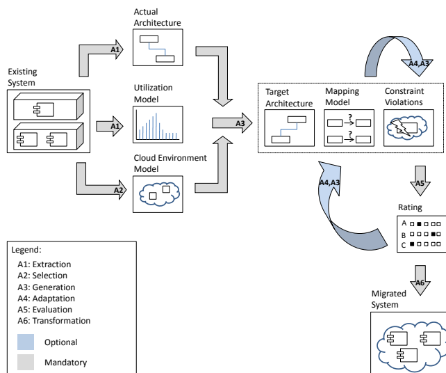
Figure 1. CloudMIG Overview.
