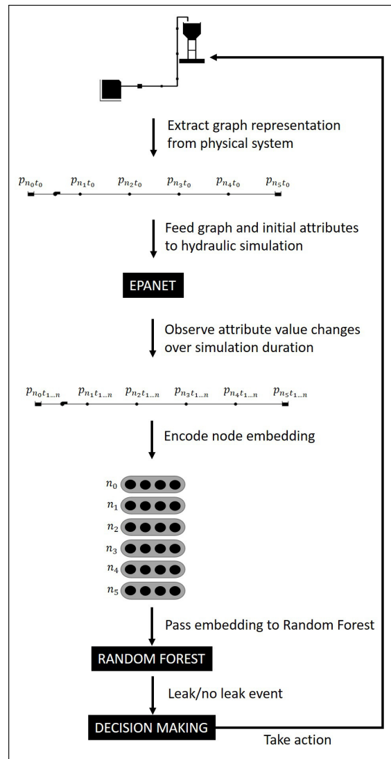
Figure 6. Process flowchart for training and executing machine.
