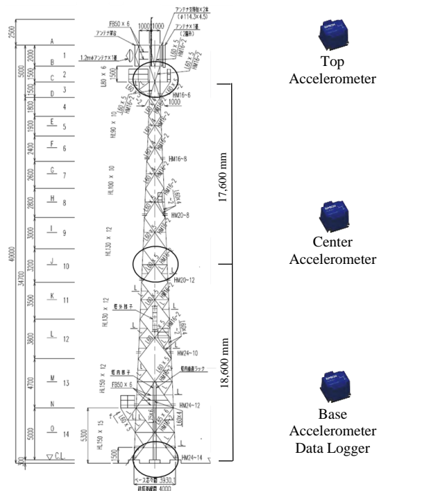
Figure 1. Steel tower structure and sensor location.
