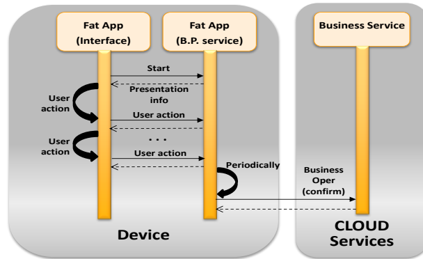
Figure 6. Fat client workflow.
