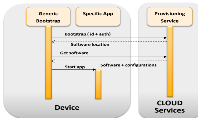
Figure 10. Provisioning workflow.
