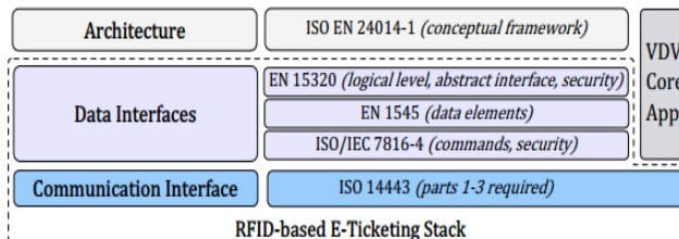
Figure 7. Standards to implement thin device concept.
