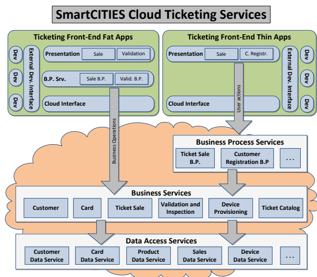
Figure 1. Cloud Ticketing Architecture.
