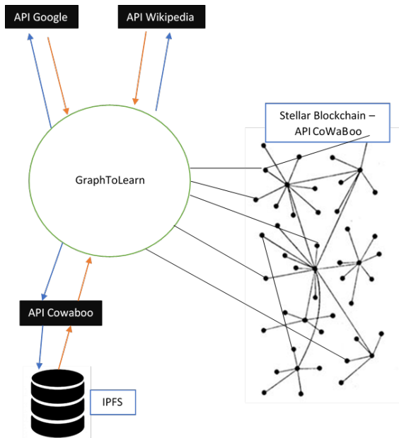
Figure 17. The GraphToLearn initial architecture
