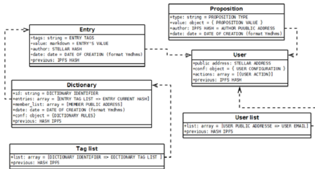
Figure 1. The connections between the CoWaBoo protocol objects
