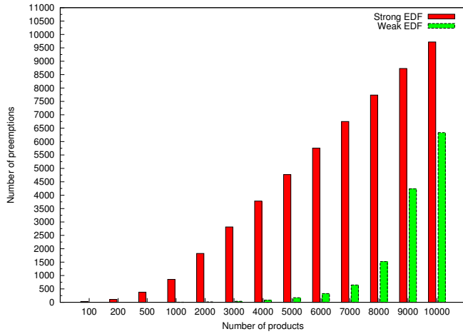
Figure 21: Number of preemptions for strong and weak EDF.
