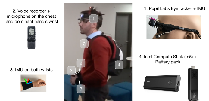
Figure 1. Recording setup for each participant includes an eyetracker connected to a small recording computer. Additional sensors: IMU on both arms and head, microphone on the wrist and at the chest.
