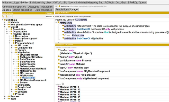
Figure 2. AMMACHINE Class in AMO ontology
